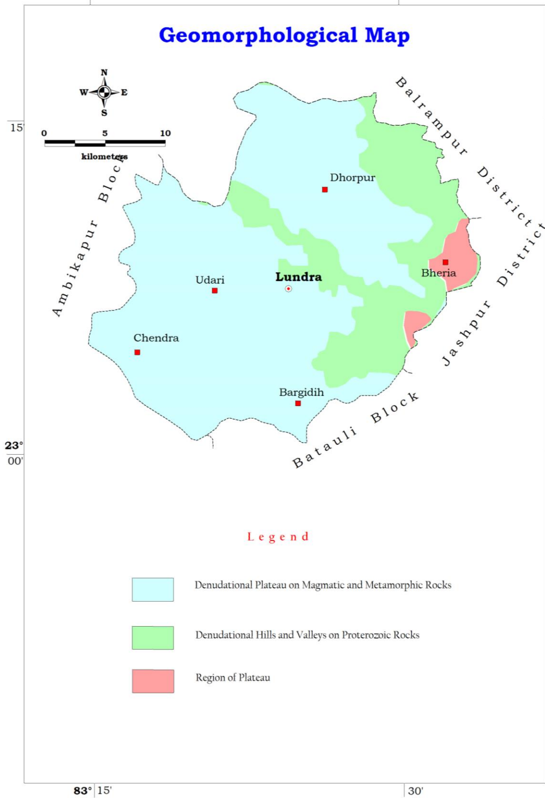
Figure 2 Geomorphology Map of Lundra Block
